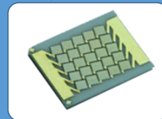
Multiple LED ceramic array built on alumina submount with AgENIG metallization and AuSn selective plating.
